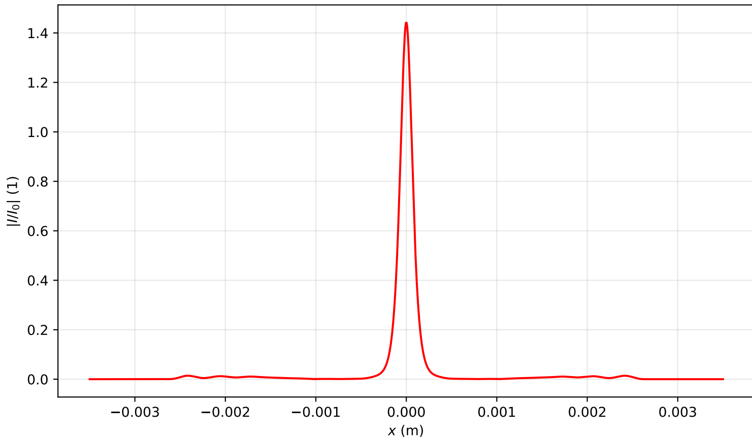
Intensity profile I(x, y = 0, z = 2.229)/I_0 , P_{in}=9.0P_{cr} , artificial time
